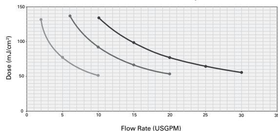
PRO10, PRO20, & PRO30 Dose Response Curves
